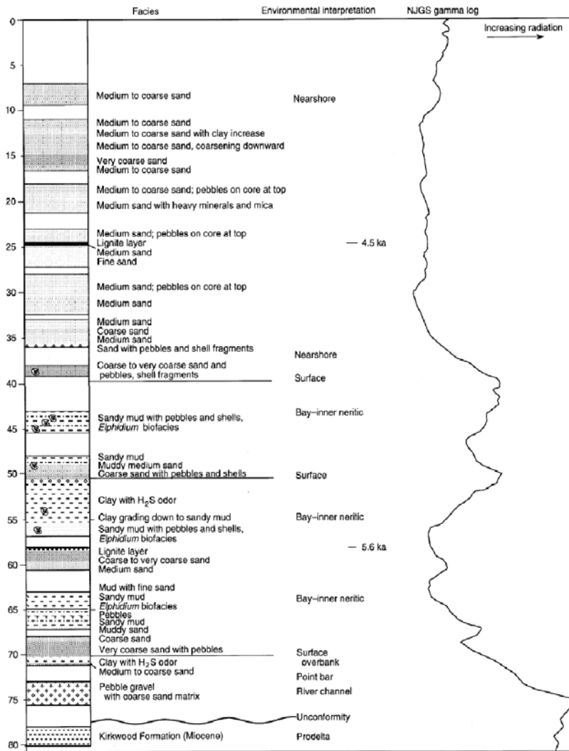
Figure 3.4: Cape May Formation lithostratigraphy, sequences, and New Jersey Geological Survey (NJGS) gamma log.
