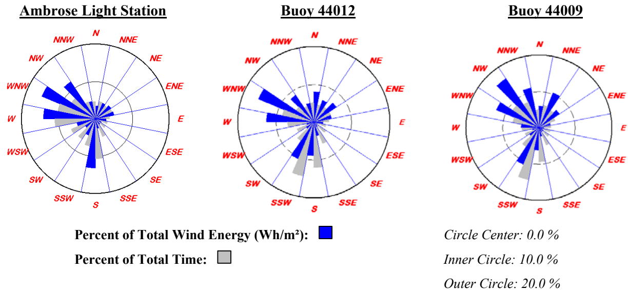
Figure 3.12: Wind Roses
